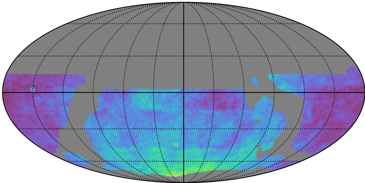
weather_cloudso8v3.4_10yrs WFD: Parallax Coverage @ 22.4
