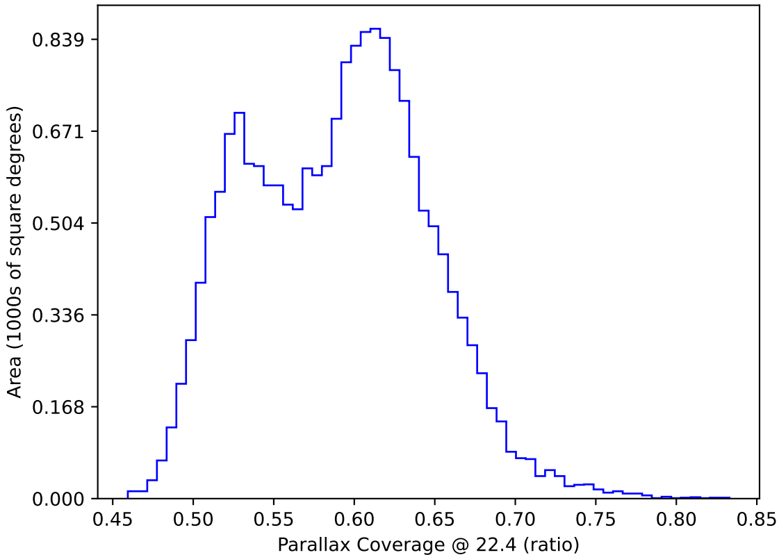
weather_cloudso8v3.4_10yrs WFD: Parallax Coverage @ 22.4
