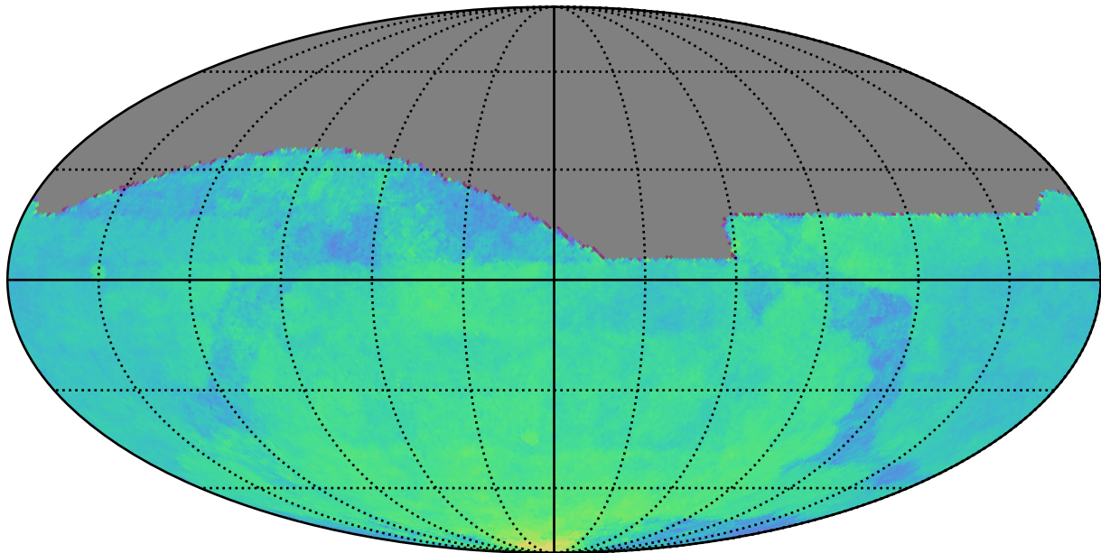
weather_cloudso8v3.4_10yrs All sky: Parallax Coverage @ 22.4
