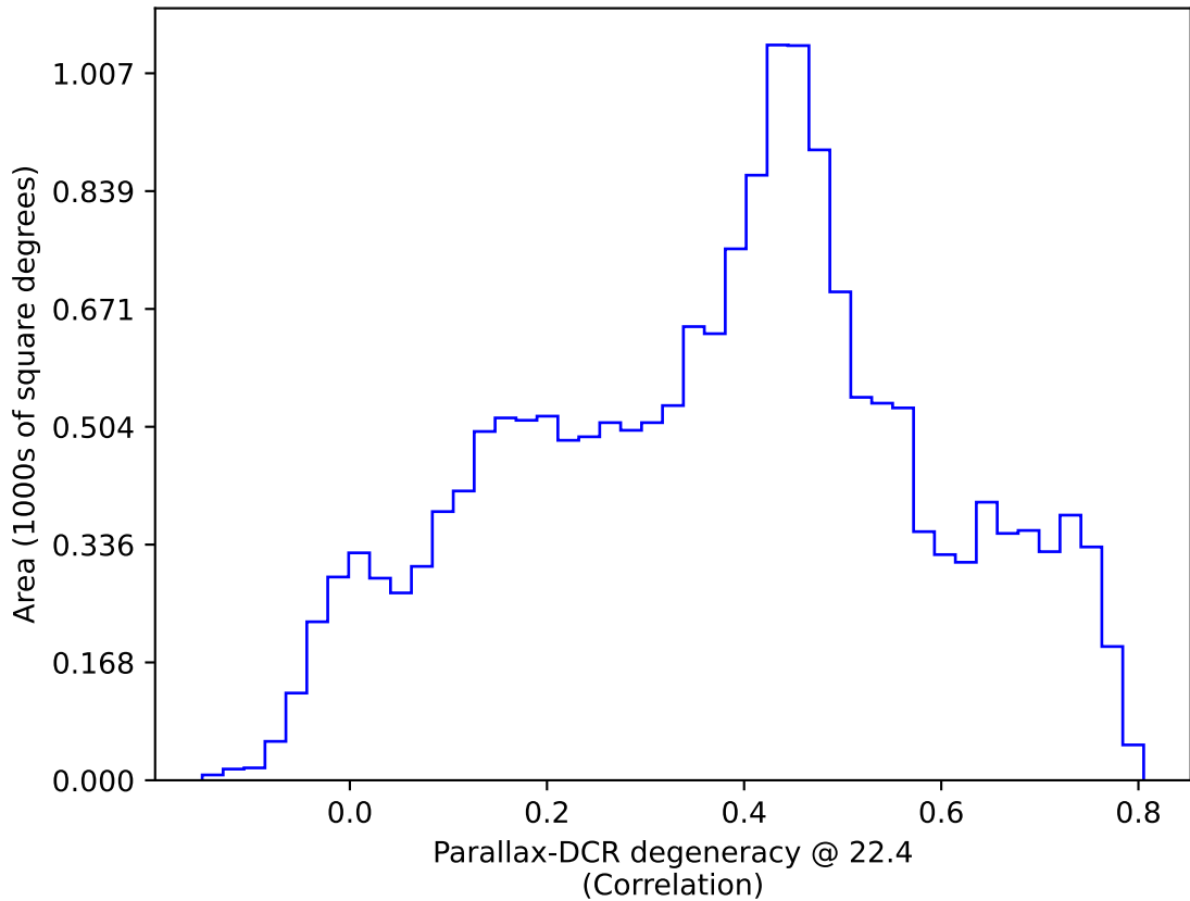
weather_cloudso8v3.4_10yrs WFD: Parallax-DCR degeneracy @ 22.4
