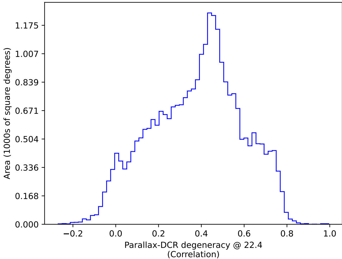
weather_cloudso8v3.4_10yrs All sky: Parallax-DCR degeneracy @ 22.4
