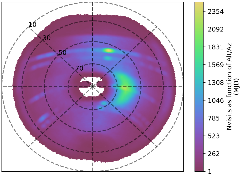
weather_cloudso8v3.4_10yrs z band: Nvisits as function of Alt/Az
