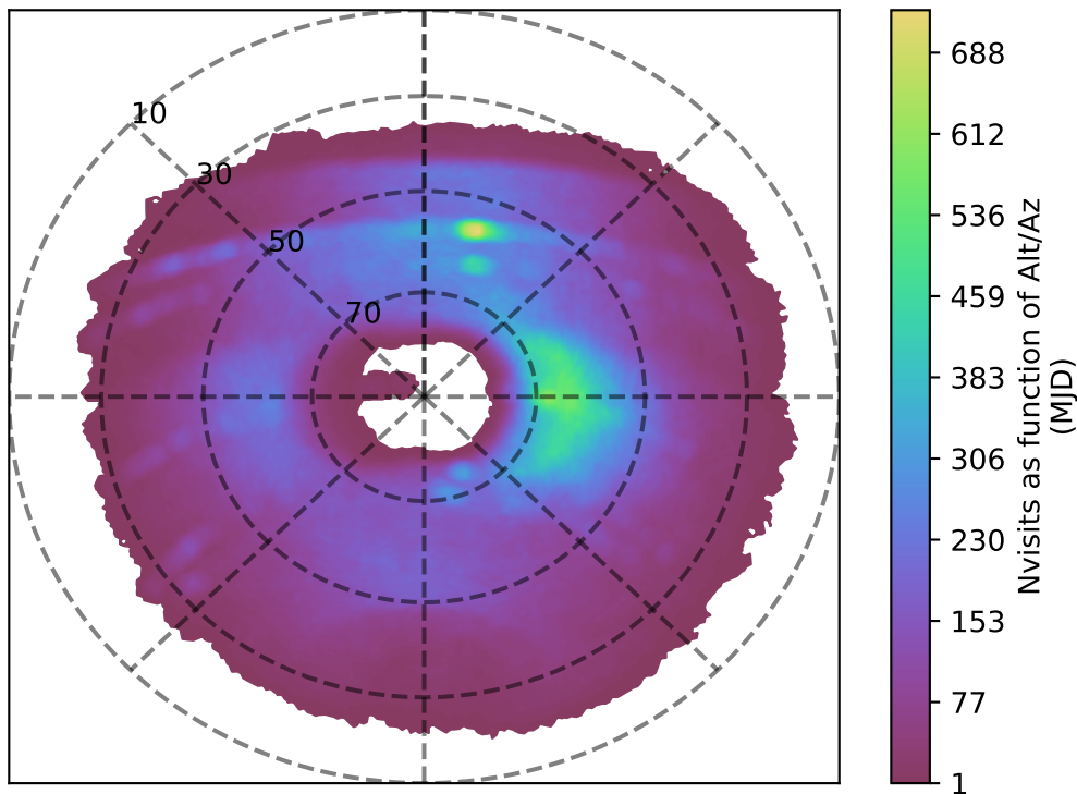
weather_cloudso8v3.4_10yrs u band: Nvisits as function of Alt/Az
