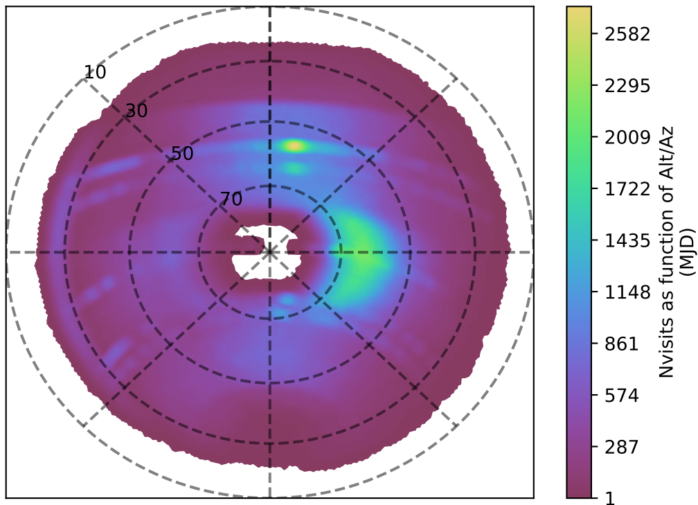
weather_cloudso8v3.4_10yrs r band: Nvisits as function of Alt/Az
