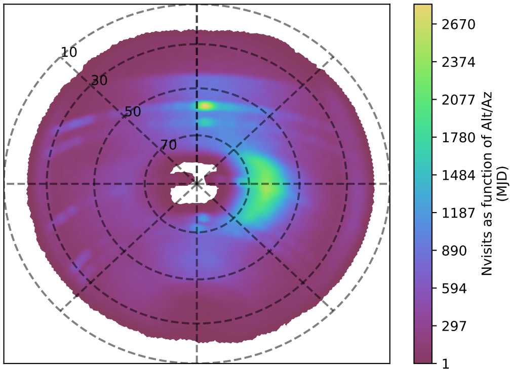
weather_cloudso8v3.4_10yrs i band: Nvisits as function of Alt/Az
