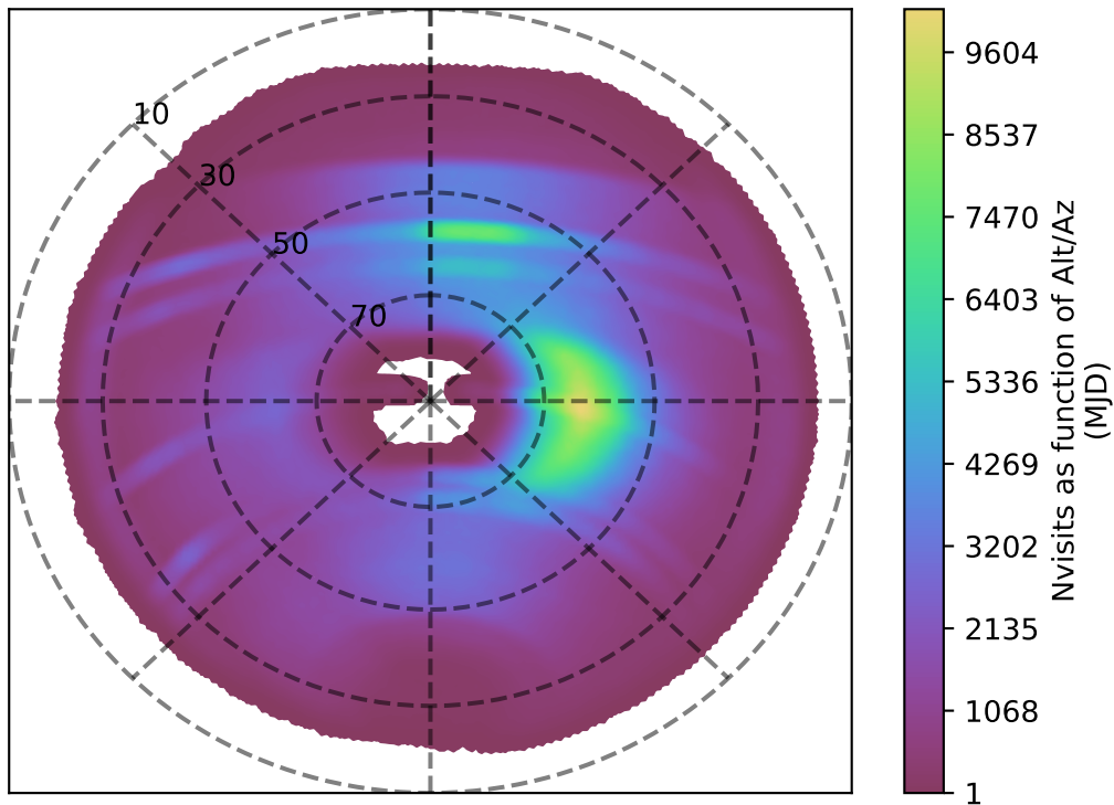
weather_cloudso8v3.4_10yrs all bands: Nvisits as function of Alt/Az
