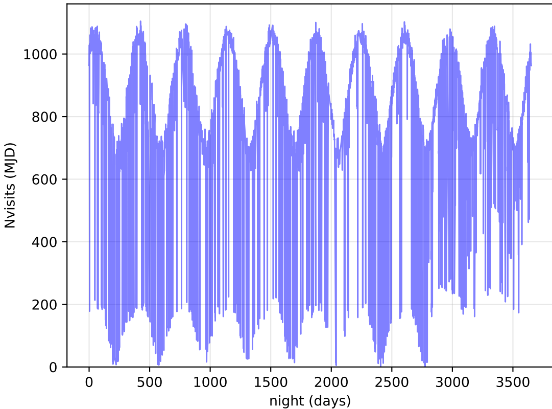
weather_cloudso8v3.4_10yrs All visits: Nvisits
