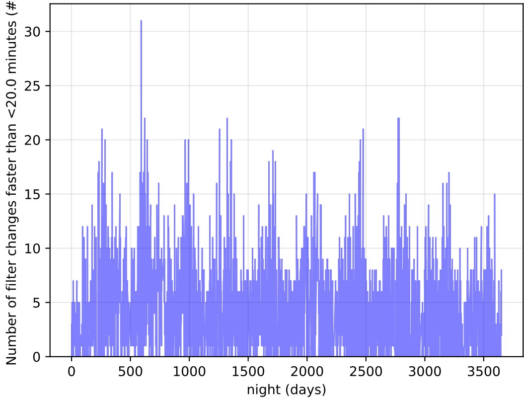
weather_cloudso8v3.4_10yrs Per Night: Number of filter changes faster than <20.0 minutes
