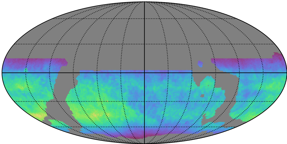
weather_cloudso8v3.4_10yrs WFD z band: Normalized Teff
