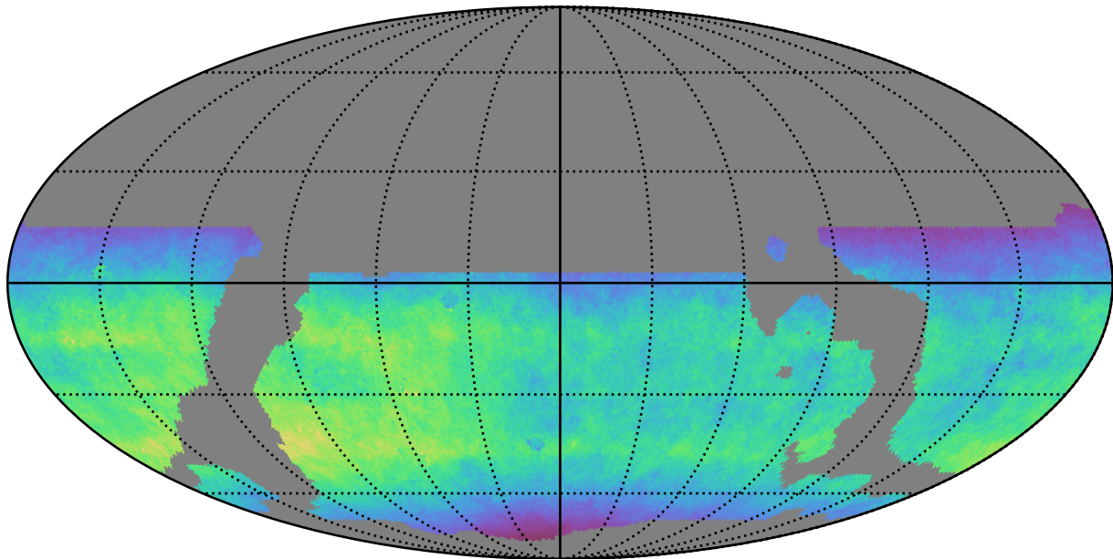
weather_cloudso8v3.4_10yrs WFD y band: Normalized Teff
