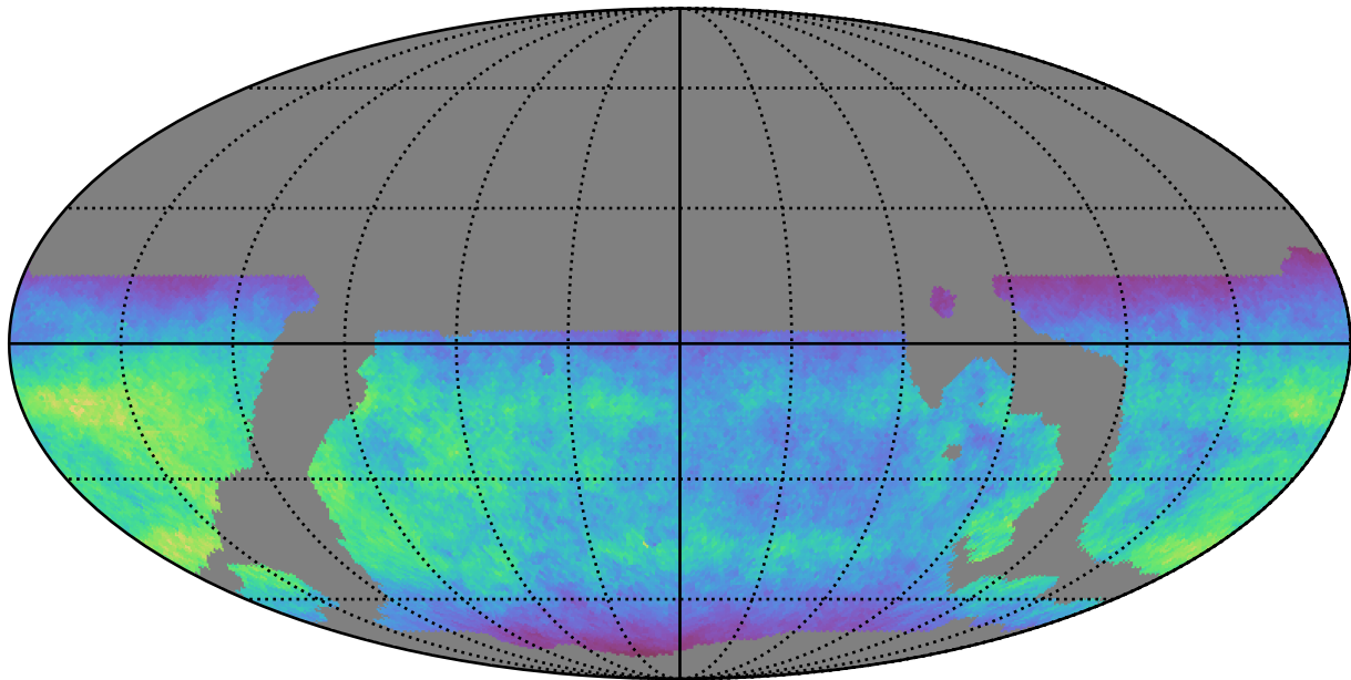
weather_cloudso8v3.4_10yrs WFD u band: Normalized Teff
