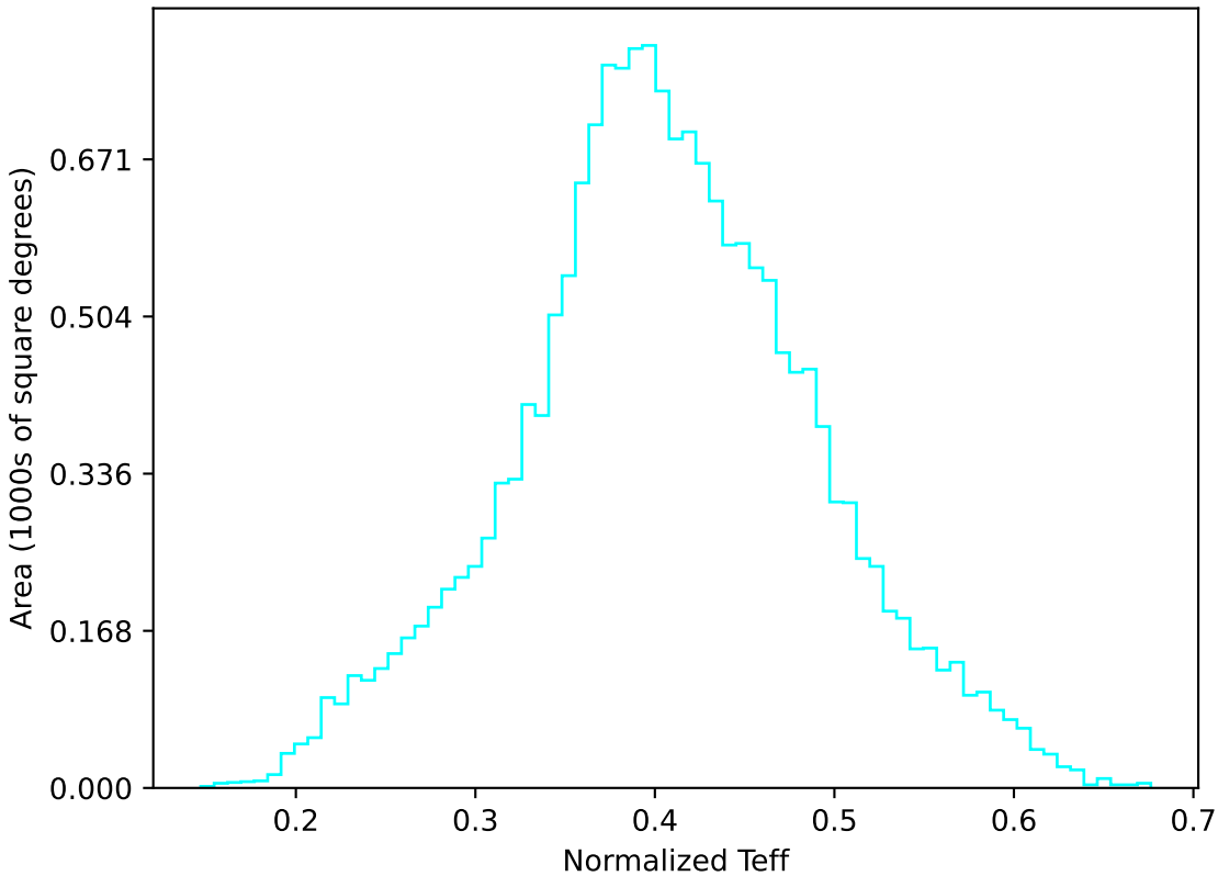
weather_cloudso8v3.4_10yrs WFD u band: Normalized Teff
