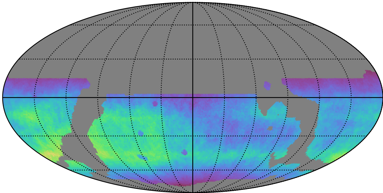
weather_cloudso8v3.4_10yrs WFD r band: Normalized Teff
