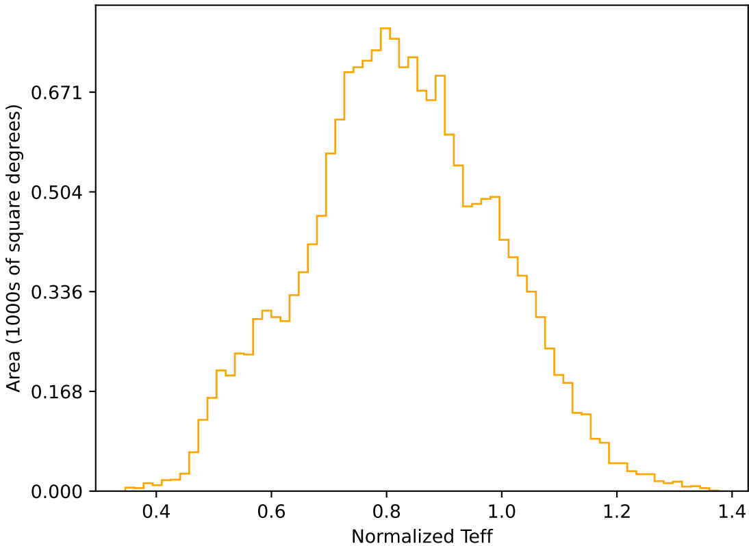
weather_cloudso8v3.4_10yrs WFD r band: Normalized Teff
