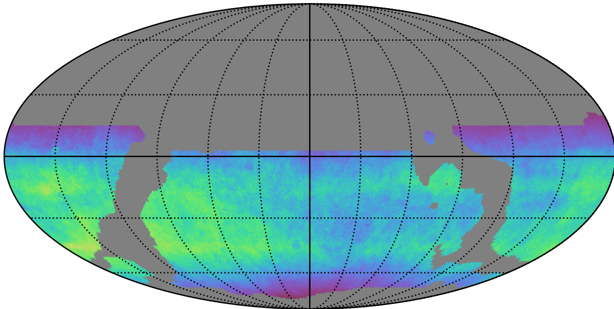
weather_cloudso8v3.4_10yrs WFD i band: Normalized Teff
