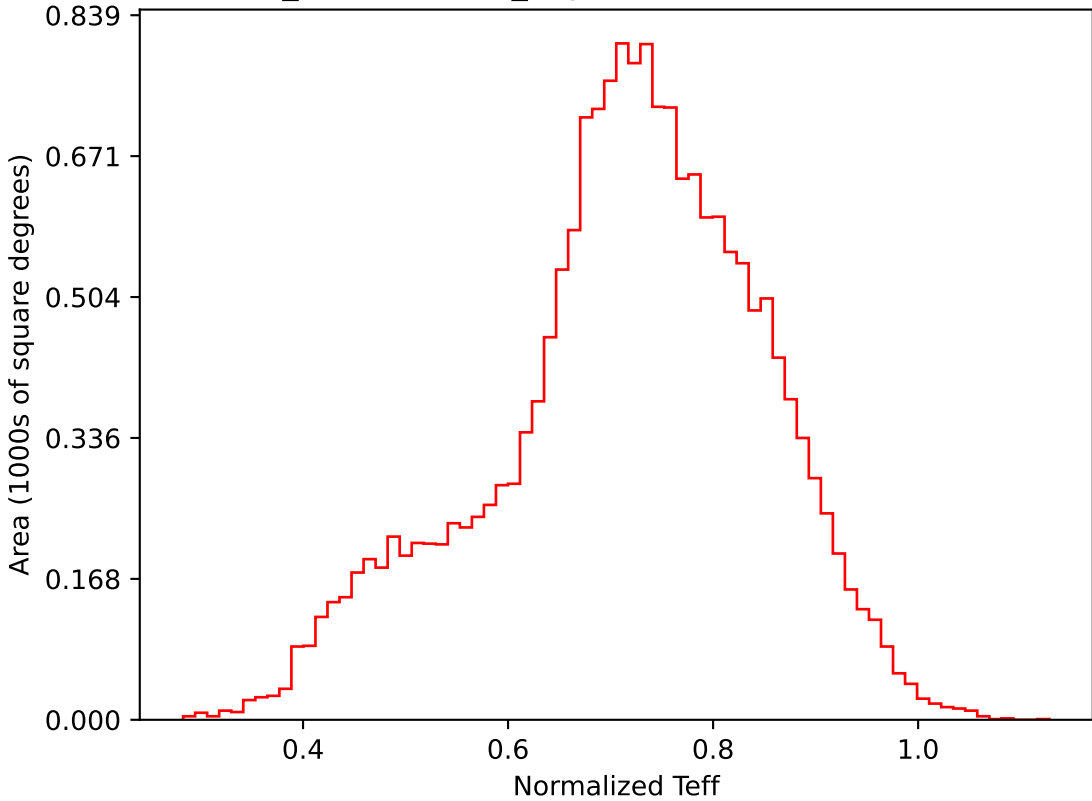
weather_cloudso8v3.4_10yrs WFD i band: Normalized Teff
