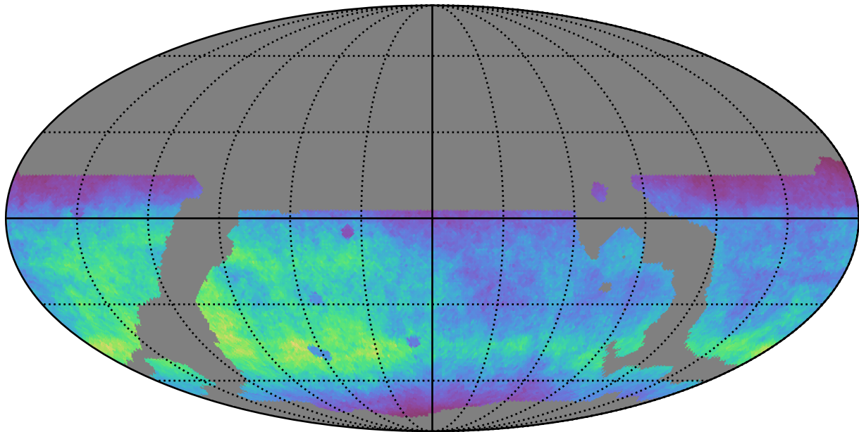
weather_cloudso8v3.4_10yrs WFD g band: Normalized Teff
