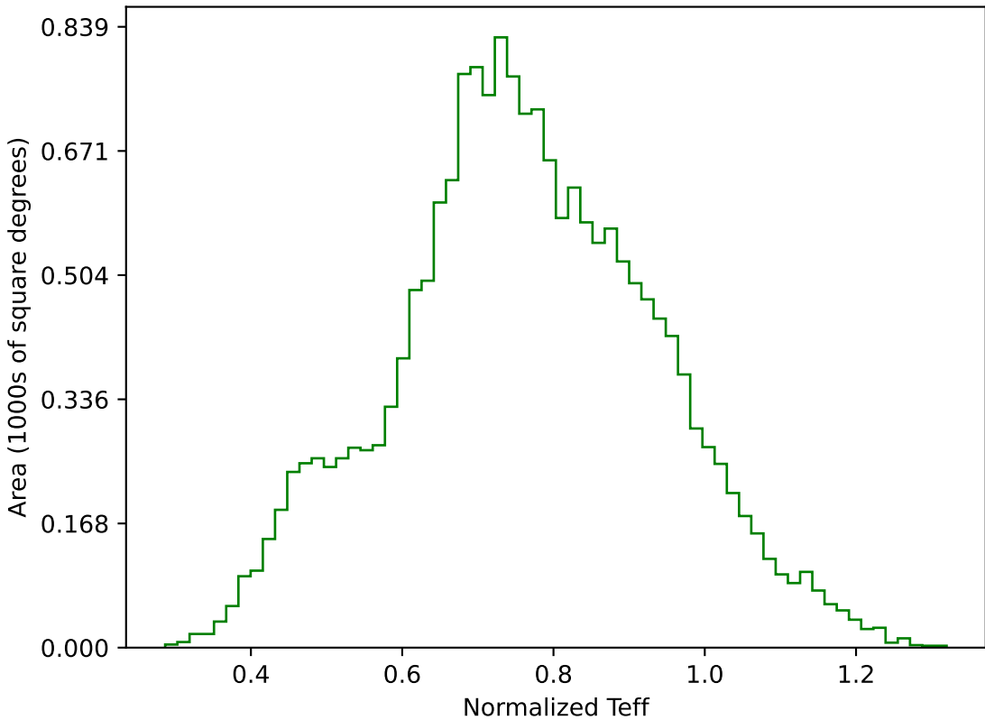
weather_cloudso8v3.4_10yrs WFD g band: Normalized Teff
