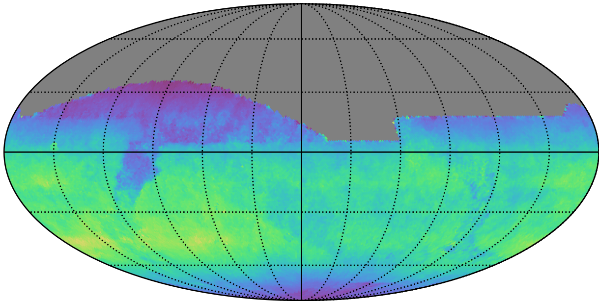
weather_cloudso8v3.4_10yrs All sky z band: Normalized Teff
