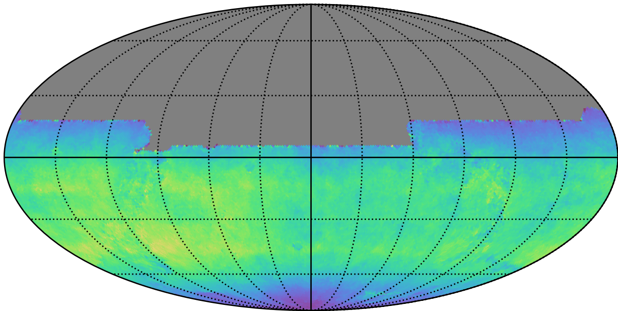
weather_cloudso8v3.4_10yrs All sky y band: Normalized Teff
