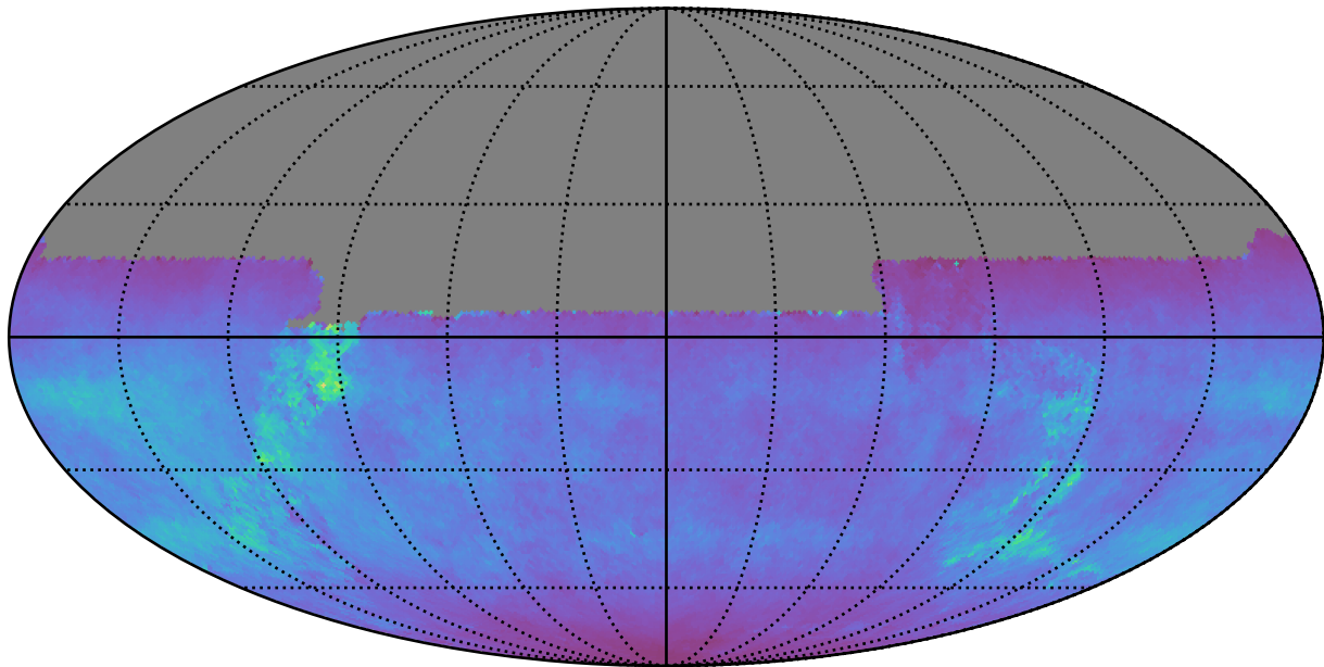
weather_cloudso8v3.4_10yrs All sky u band: Normalized Teff
