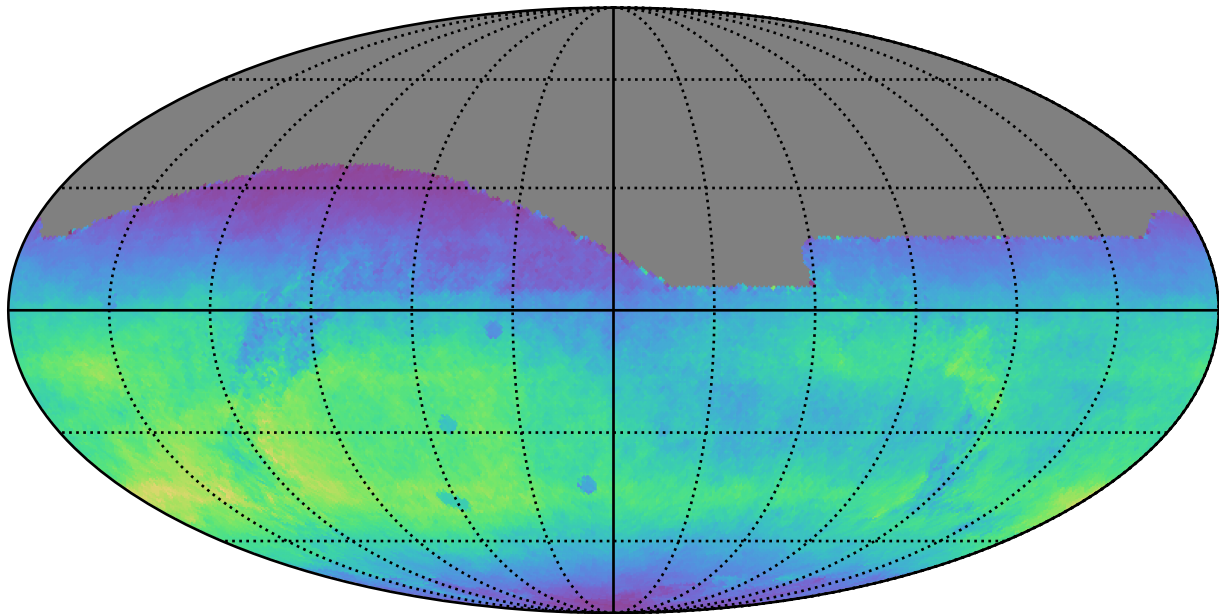
weather_cloudso8v3.4_10yrs All sky r band: Normalized Teff
