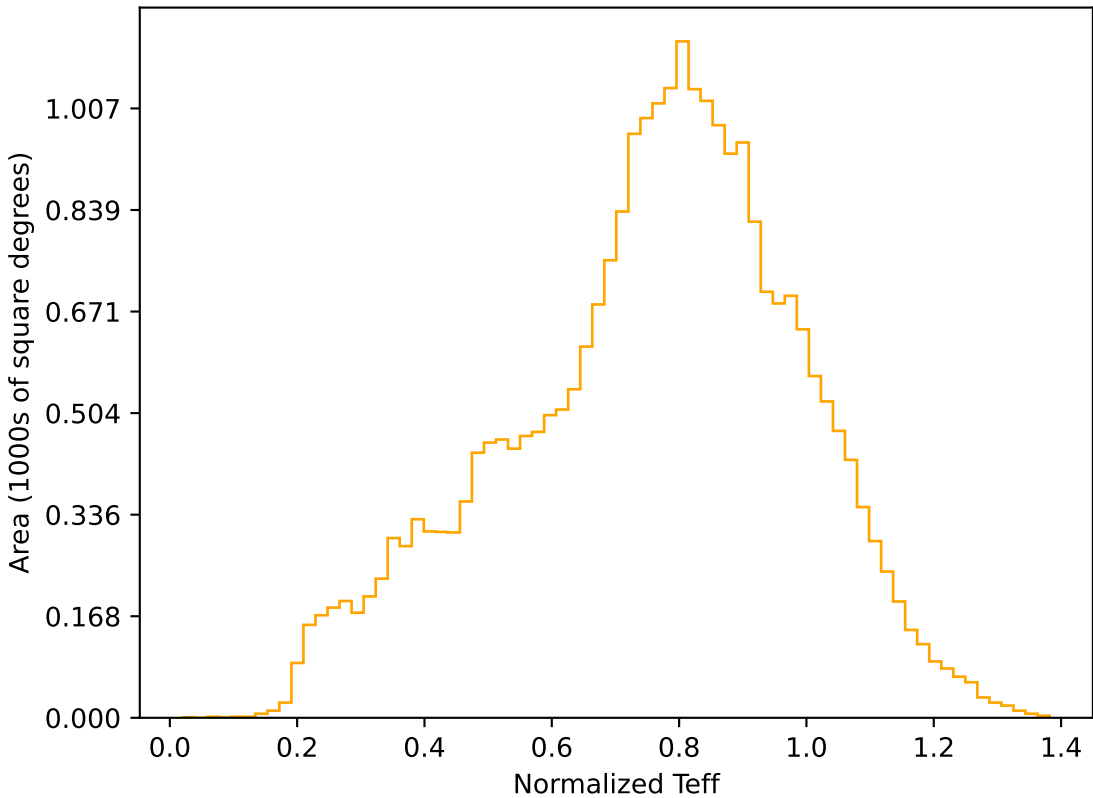
weather_cloudso8v3.4_10yrs All sky r band: Normalized Teff
