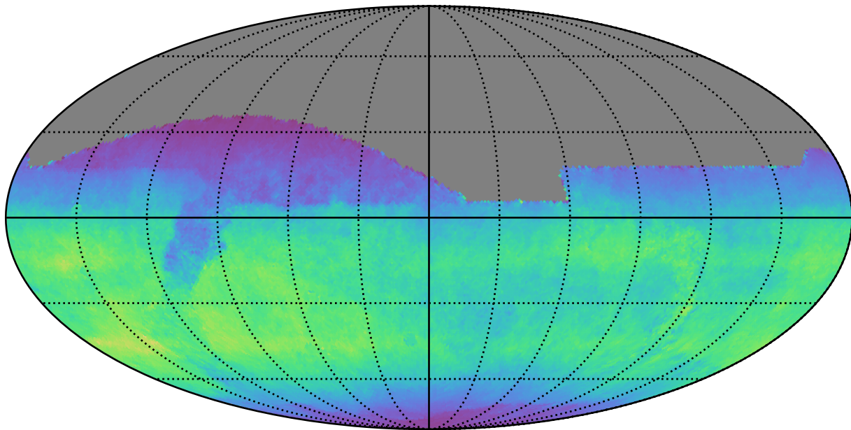
weather_cloudso8v3.4_10yrs All sky i band: Normalized Teff
