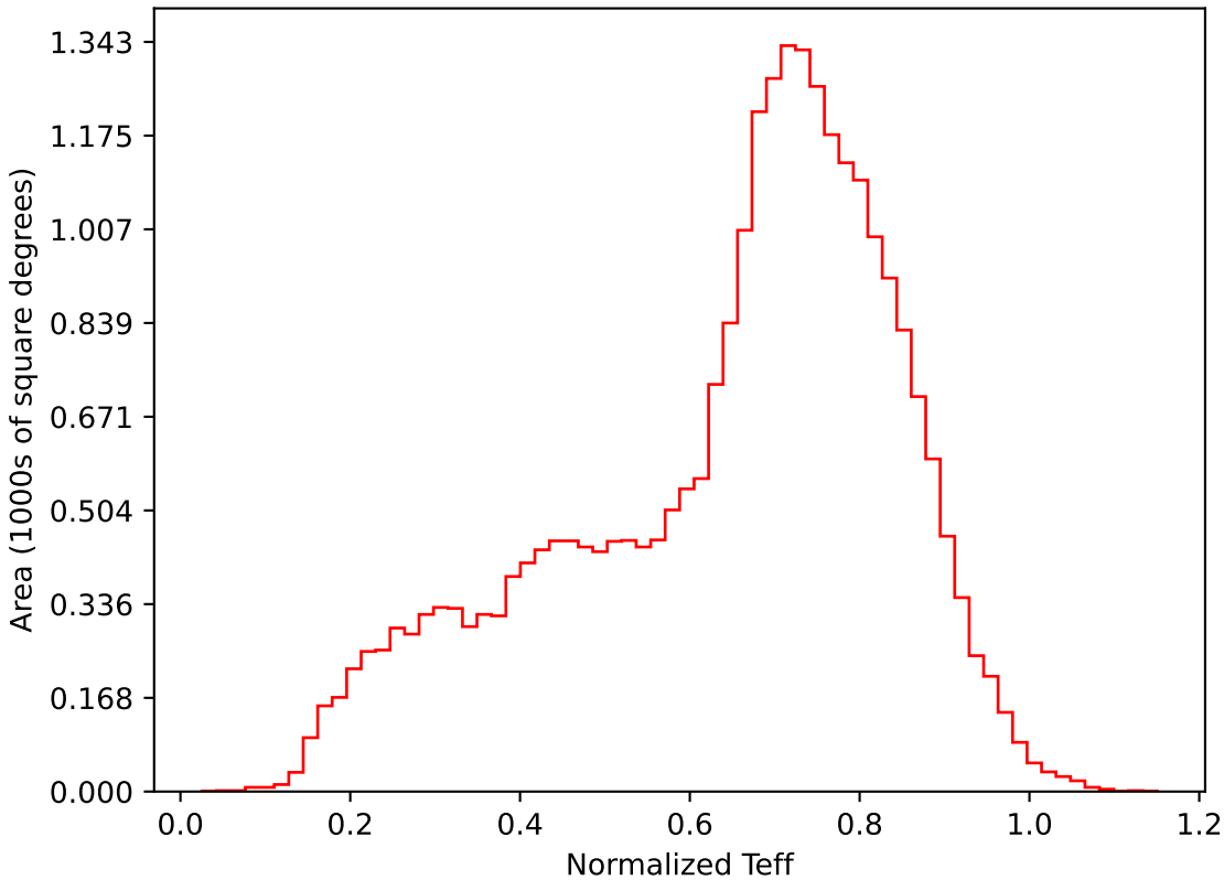
weather_cloudso8v3.4_10yrs All sky i band: Normalized Teff
