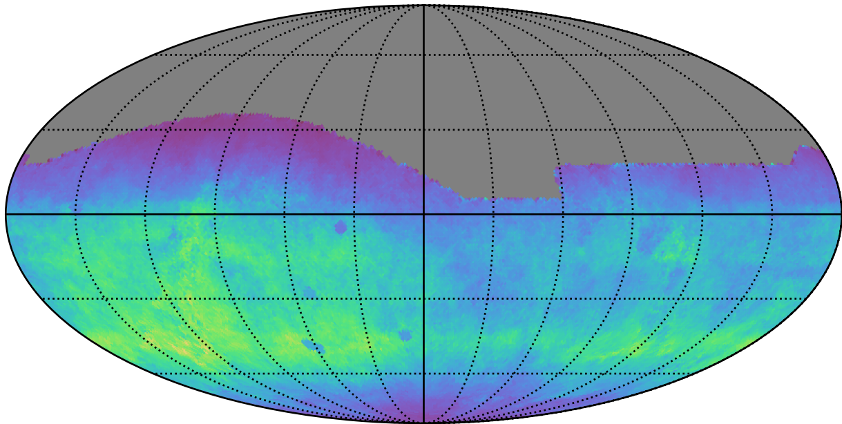
weather_cloudso8v3.4_10yrs All sky g band: Normalized Teff
