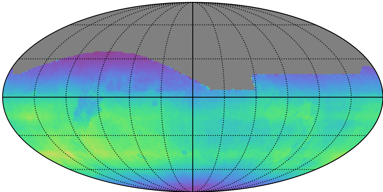
weather_cloudso8v3.4_10yrs All sky all bands: Normalized Teff
