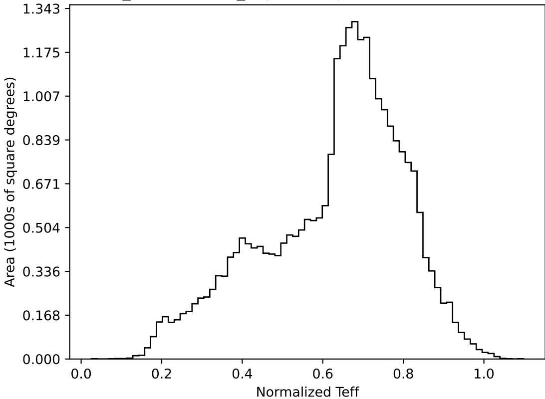
weather_cloudso8v3.4_10yrs All sky all bands: Normalized Teff
