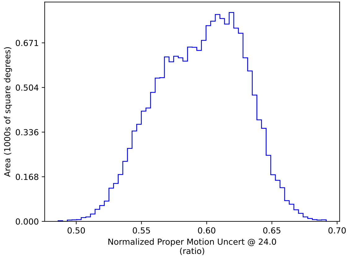
weather_cloudso8v3.4_10yrs WFD: Normalized Proper Motion Uncert @ 24.0
