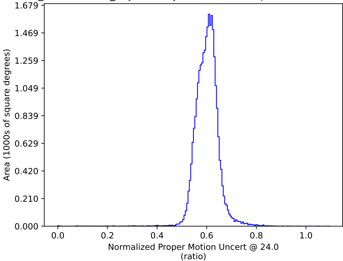
weather_cloudso8v3.4_10yrs All sky: Normalized Proper Motion Uncert @ 24.0
