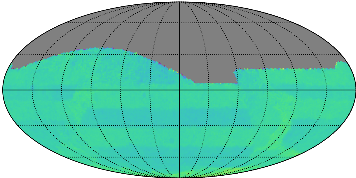
weather_cloudso8v3.4_10yrs All sky: Normalized Proper Motion Uncert @ 20.5
