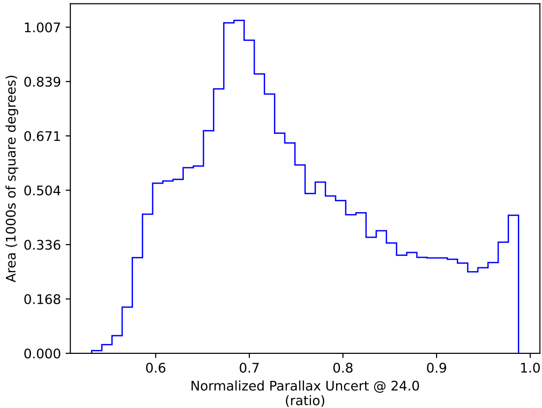
weather_cloudso8v3.4_10yrs WFD: Normalized Parallax Uncert @ 24.0
