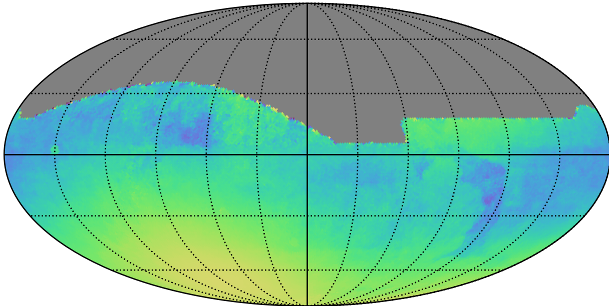
weather_cloudso8v3.4_10yrs All sky: Normalized Parallax Uncert @ 24.0
