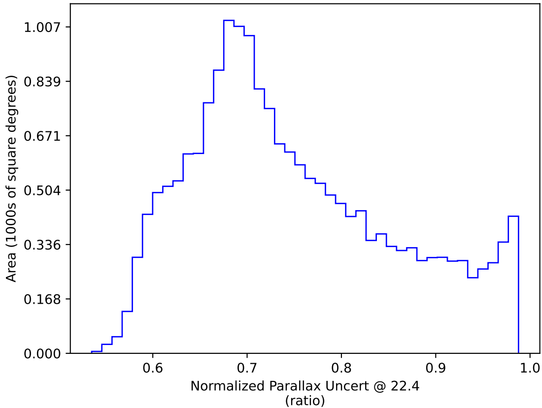
weather_cloudso8v3.4_10yrs WFD: Normalized Parallax Uncert @ 22.4
