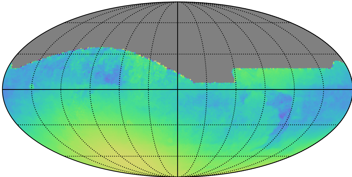
weather_cloudso8v3.4_10yrs All sky: Normalized Parallax Uncert @ 22.4
