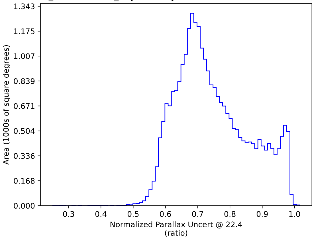
weather_cloudso8v3.4_10yrs All sky: Normalized Parallax Uncert @ 22.4
