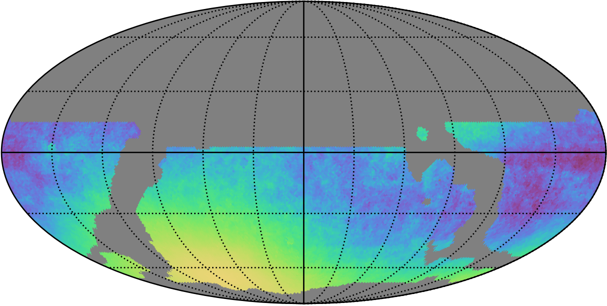
weather_cloudso8v3.4_10yrs WFD y band only: Normalized Parallax Uncert @ 21.3
