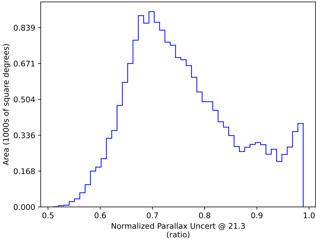
weather_cloudso8v3.4_10yrs WFD y band only: Normalized Parallax Uncert @ 21.3
