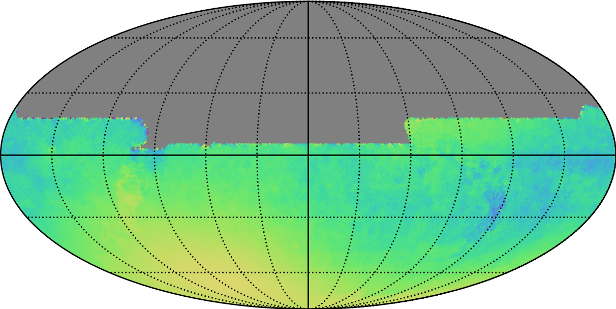
weather_cloudso8v3.4_10yrs All sky y band only: Normalized Parallax Uncert @ 21.3
