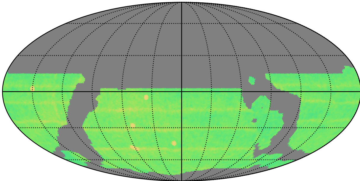
weather_cloudso8v3.4_10yrs WFD all bands: N Unique Nights
