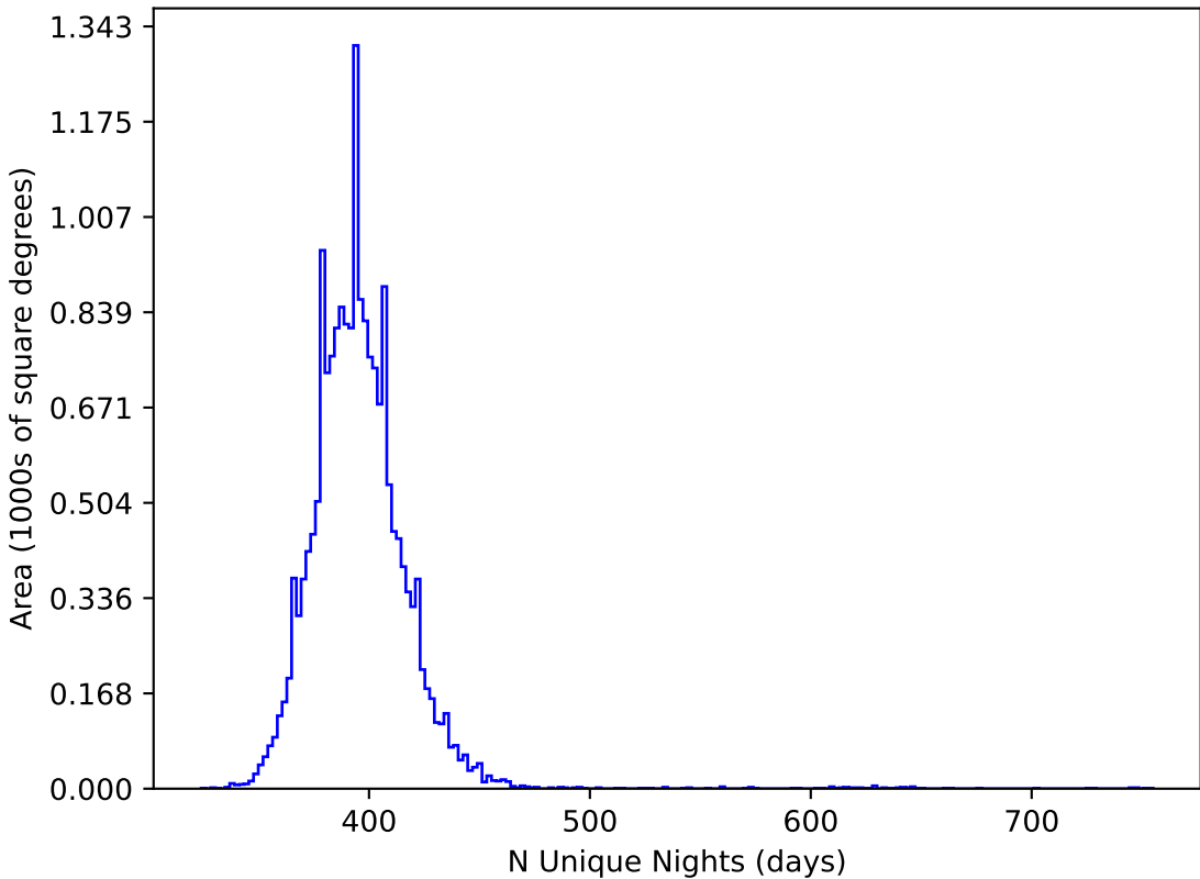
weather_cloudso8v3.4_10yrs WFD all bands: N Unique Nights
