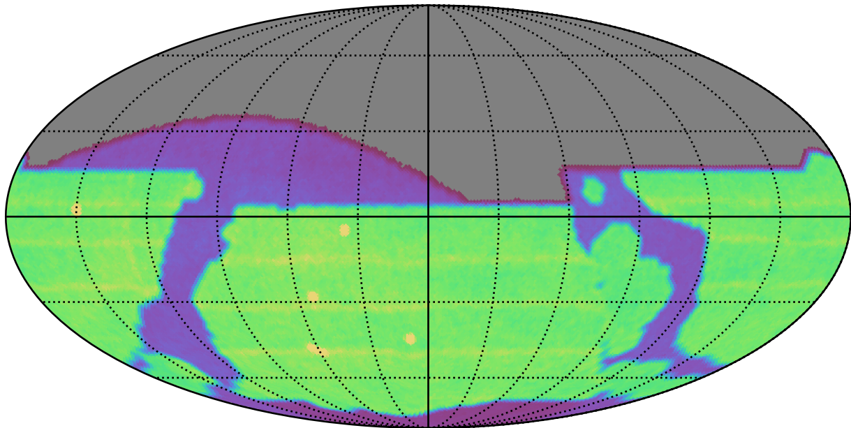
weather_cloudso8v3.4_10yrs All sky all bands: N Unique Nights
