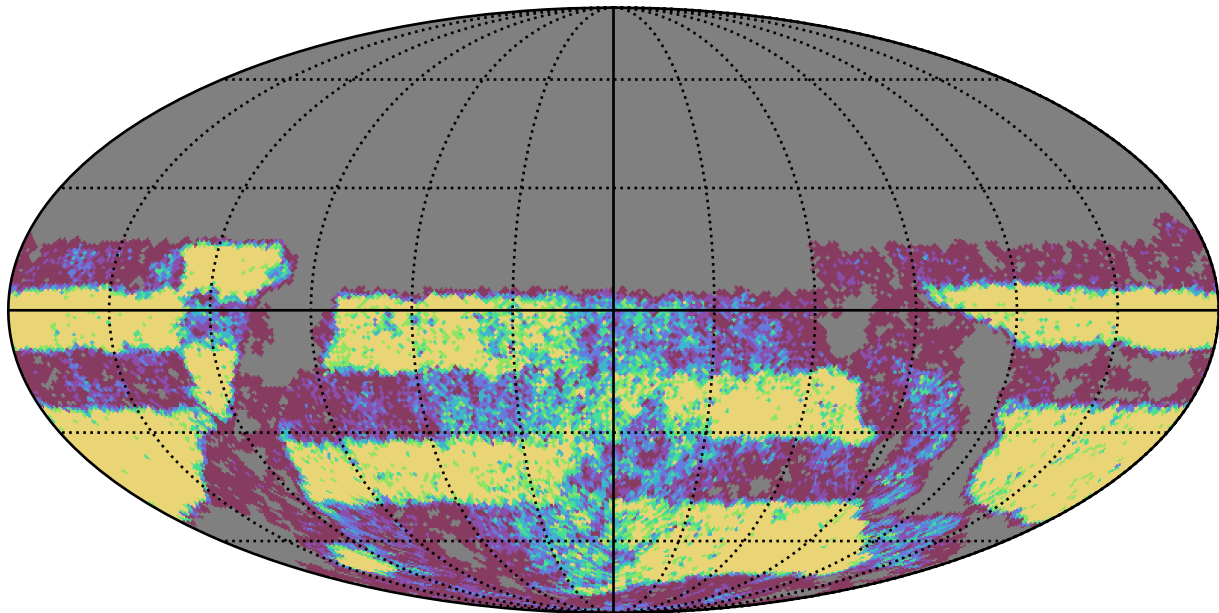
weather_cloudso8v3.4_10yrs Yr 3-4 u band: NVisits
