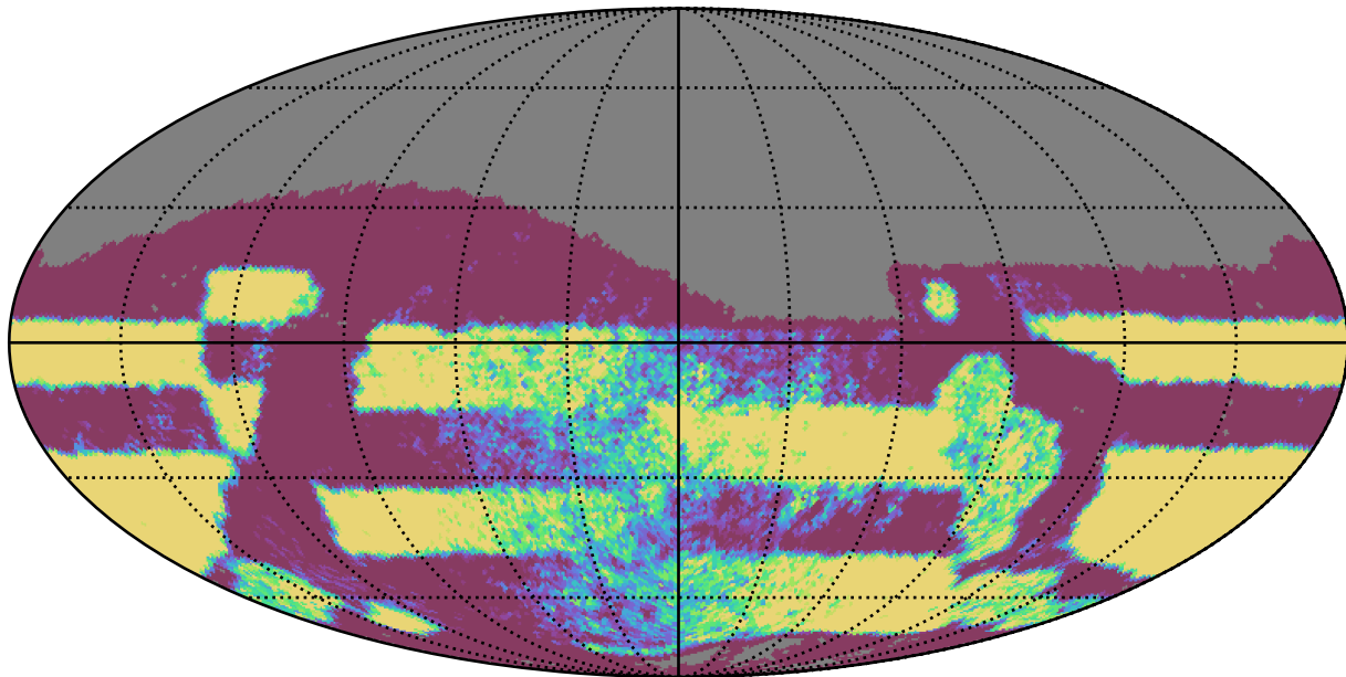
weather_cloudso8v3.4_10yrs Yr 3-4 r band: NVisits
