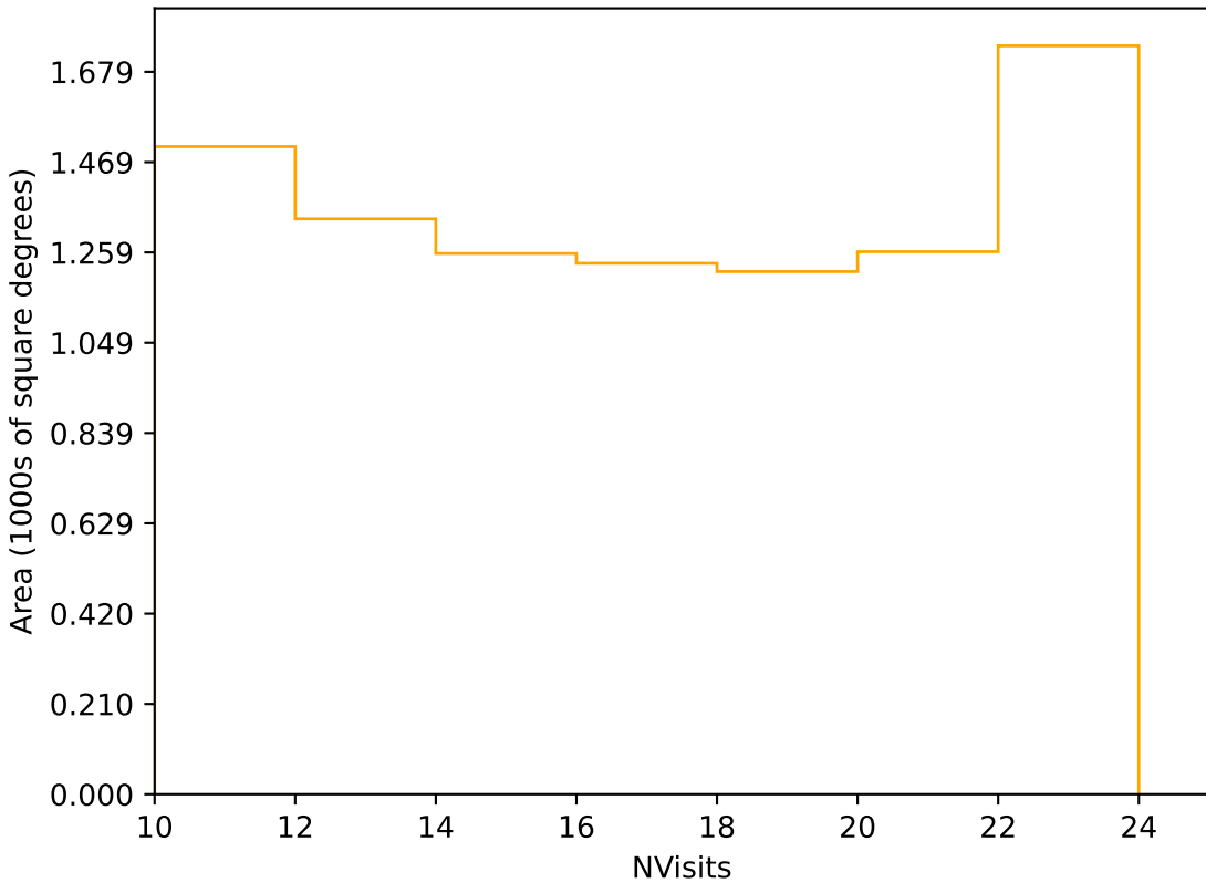
weather_cloudso8v3.4_10yrs Yr 3-4 r band: NVisits
