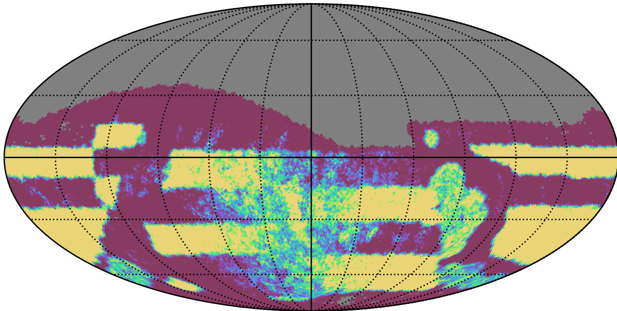
weather_cloudso8v3.4_10yrs Yr 3-4 i band: NVisits
